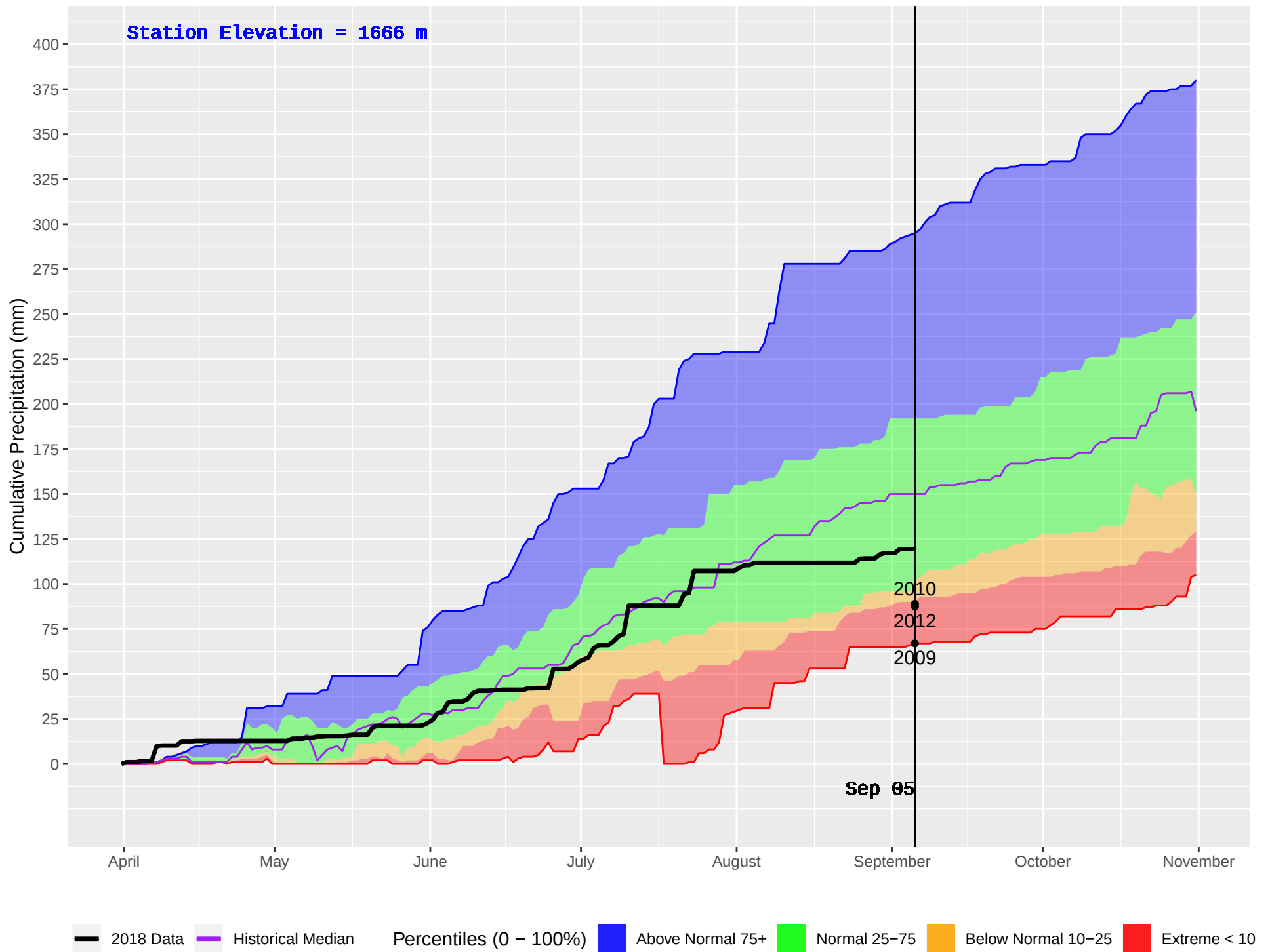
BALDFACE (221) : Historical (1992–2016) and Current (2018) Daily Cumulative Precipitation
