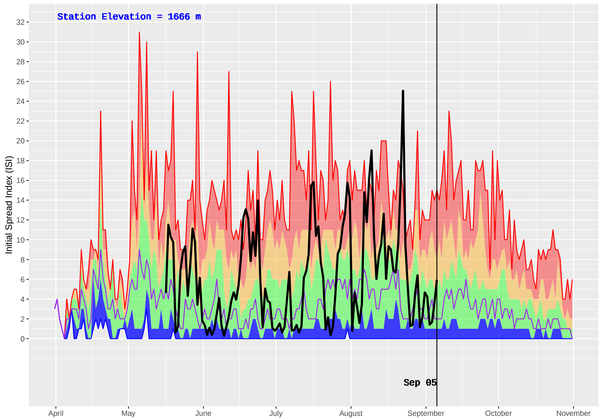
BALDFACE (221) : Historical (1992–2016) and Current (2018) Daily Initial Spread Index (ISI)
