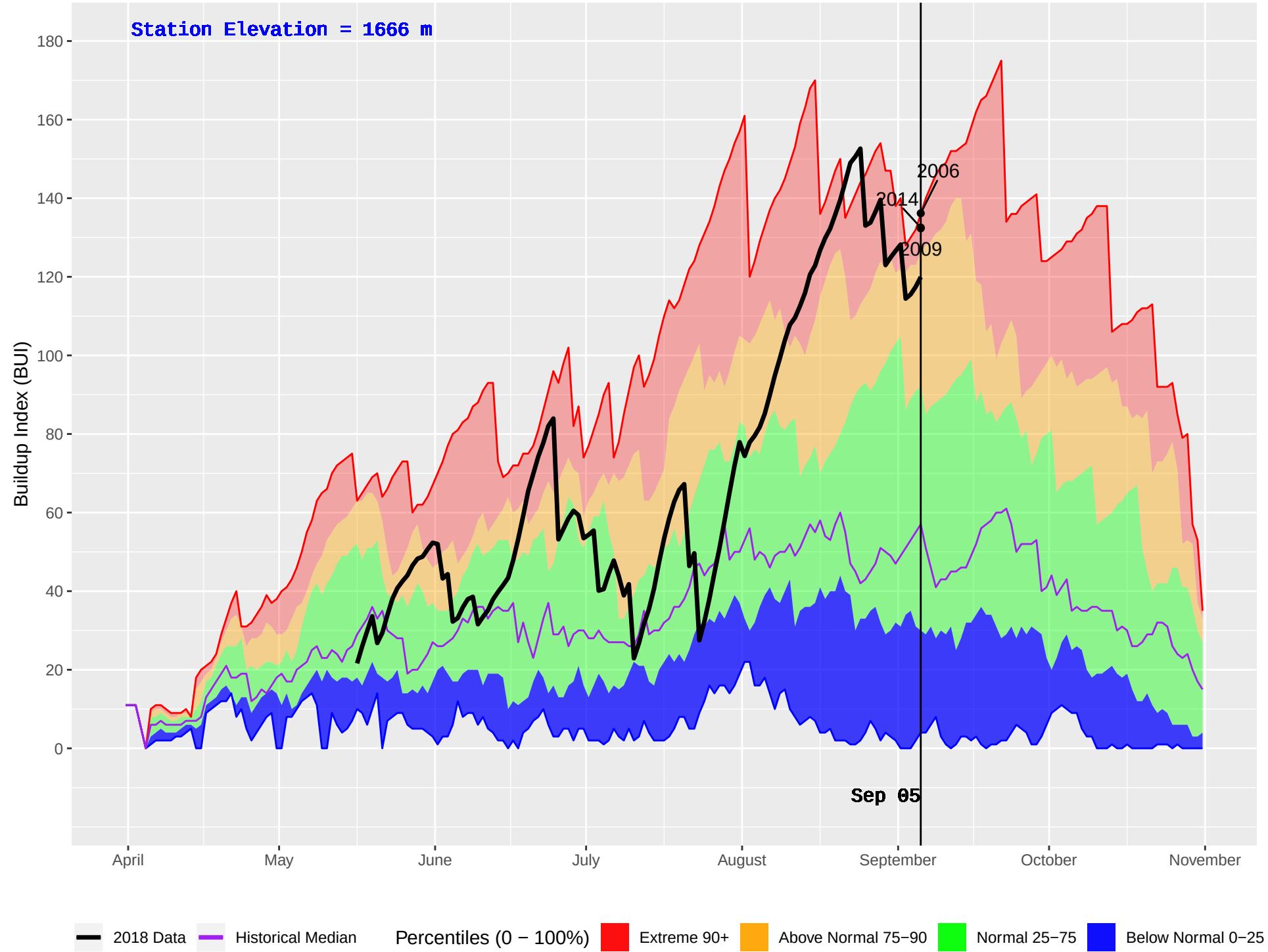
BALDFACE (221) : Historical (1992–2016) and Current (2018) Daily Buildup Index (BUI)
