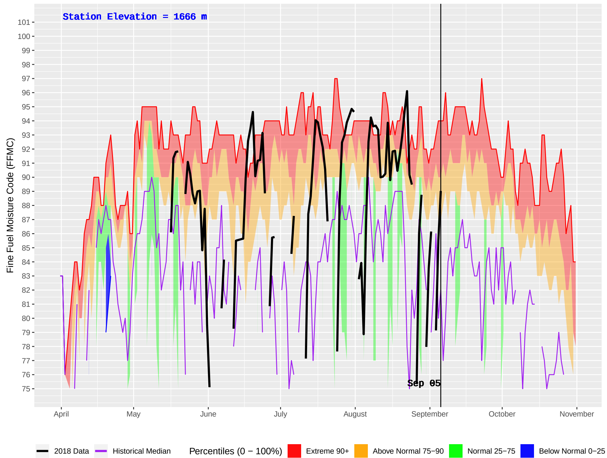
BALDFACE (221) : Historical (1992–2016) and Current (2018) Daily Fine Fuel Moisture Code (FFMC)
