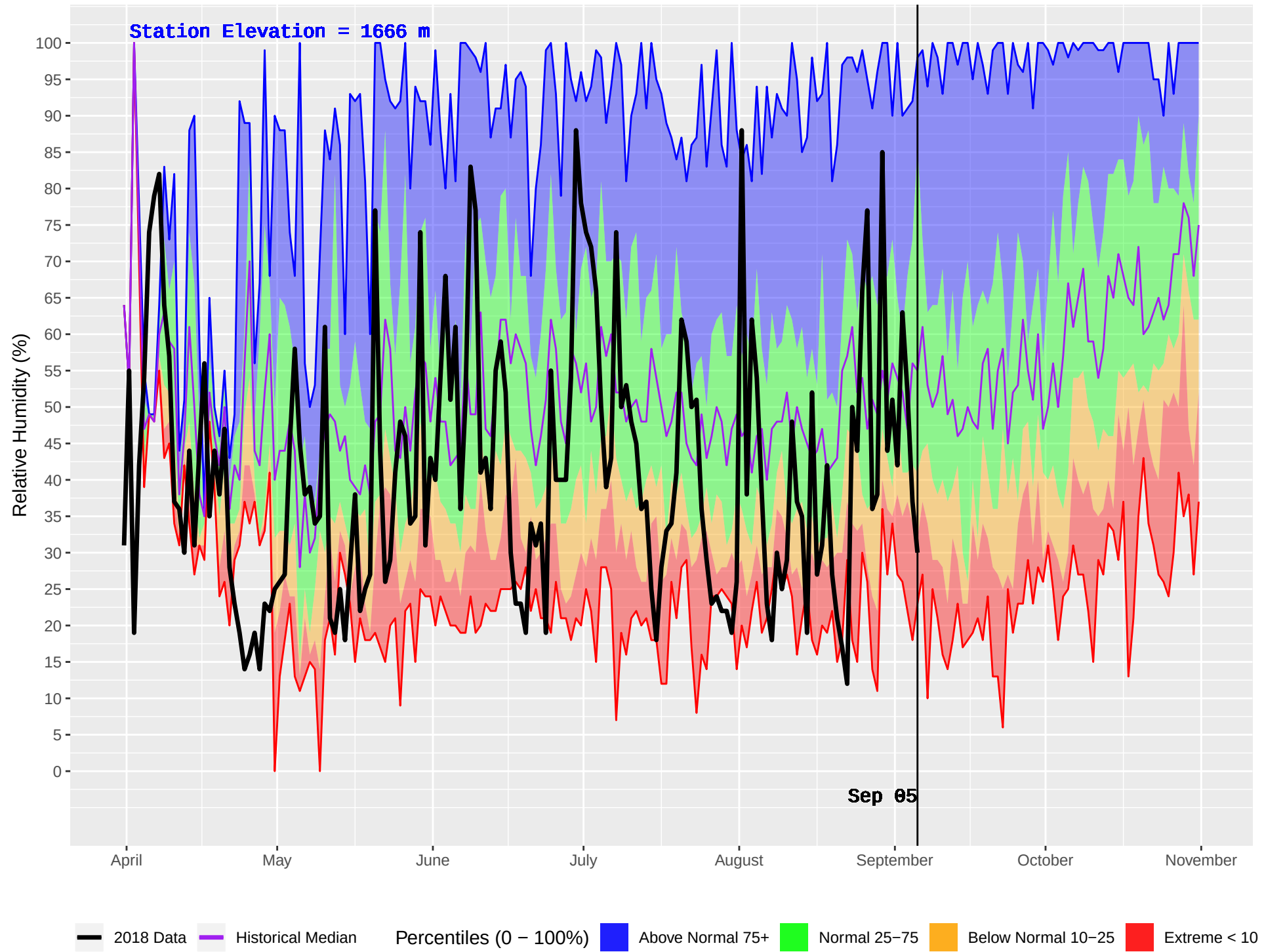
BALDFACE (221) : Historical (1992–2016) and Current (2018) Daily Relative Humidity
