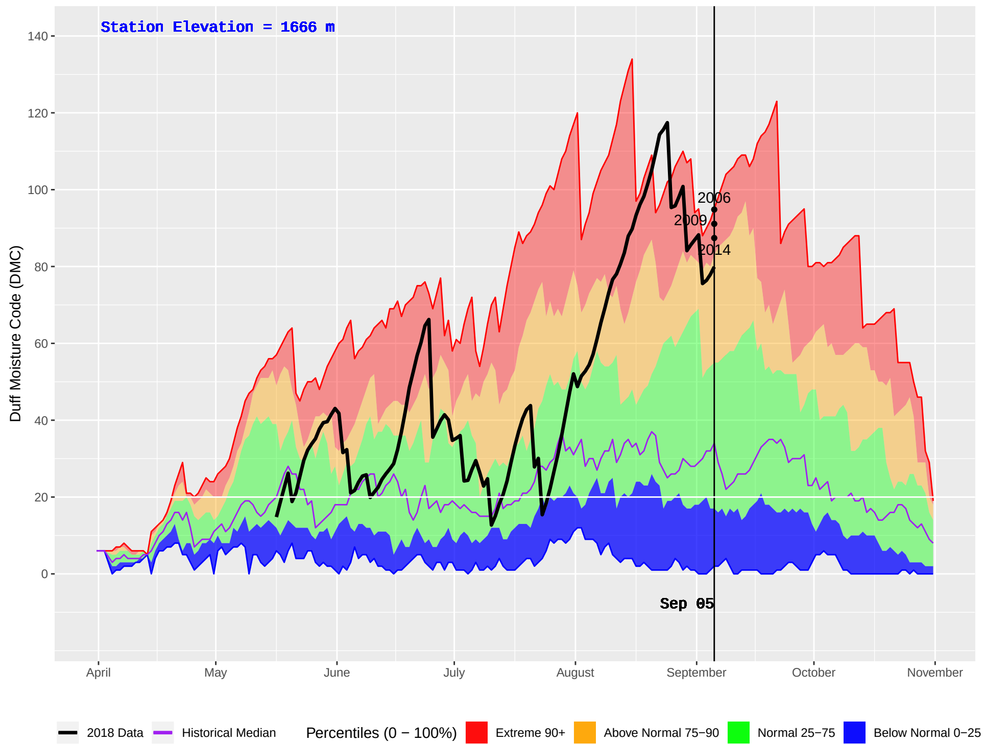
BALDFACE (221) : Historical (1992–2016) and Current (2018) Daily Duff Moisture Code (DMC)
