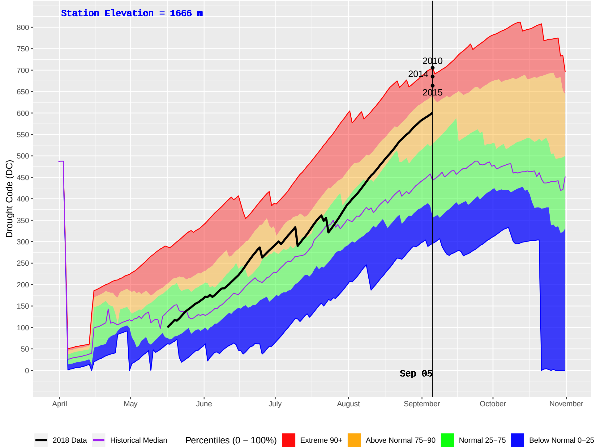
BALDFACE (221) : Historical (1992–2016) and Current (2018) Daily Drought Code (DC)
